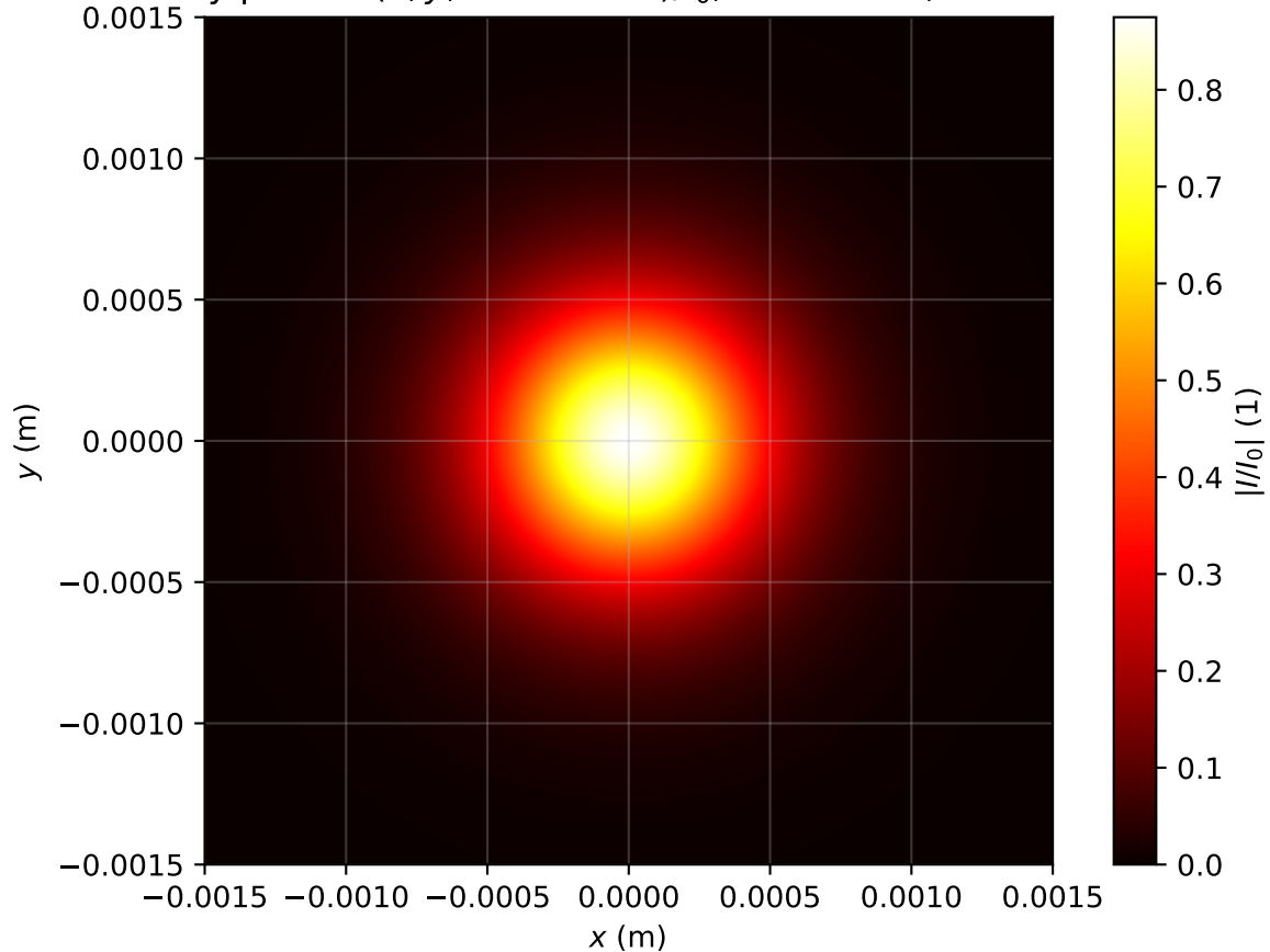
Intensity profile I(x, y, z = 2.866m)/I_0 , \text{Pin}=0.7\text{Pcr} , artificial time
